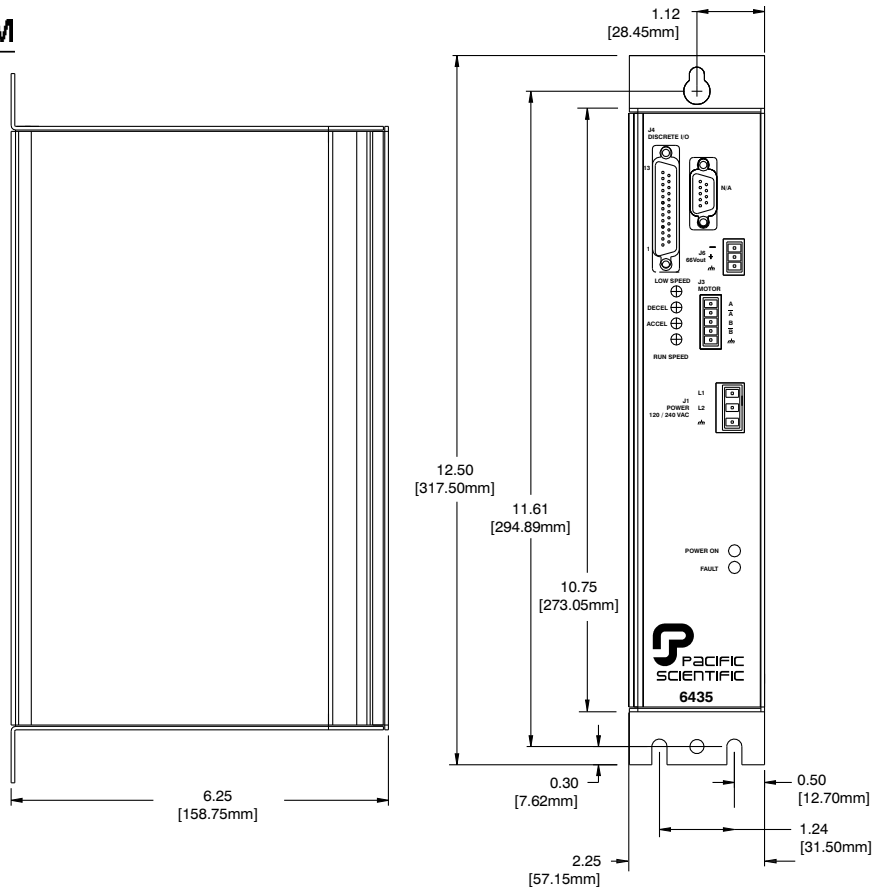
Figure 8 - 6435 Mounting Dimensions
