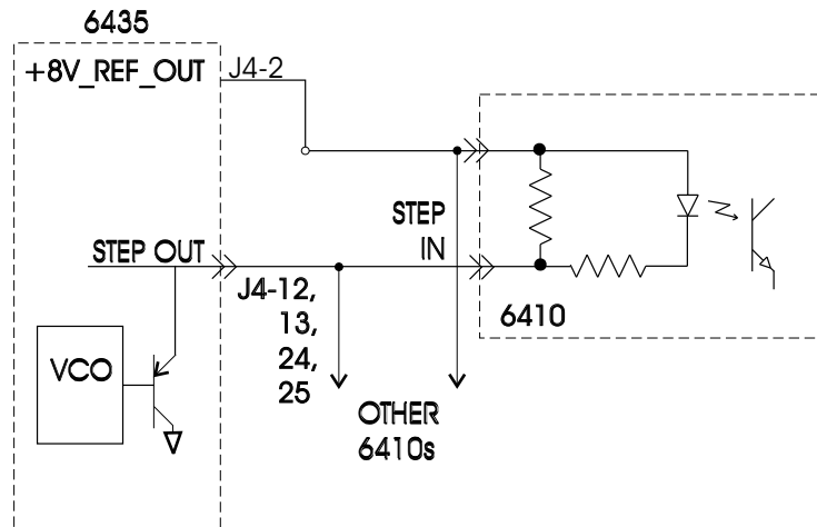
Figure 2 - External Step Pulse
